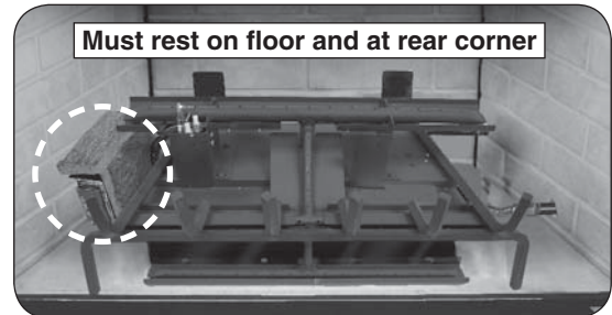
Fig. 18-1 Place heat shield (if applicable)
