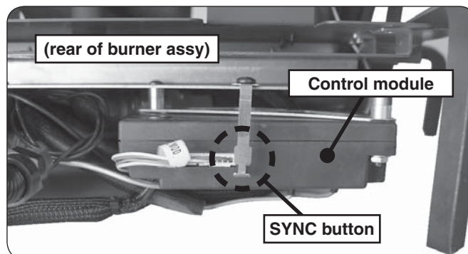
Fig. 44-2 Sync detail
