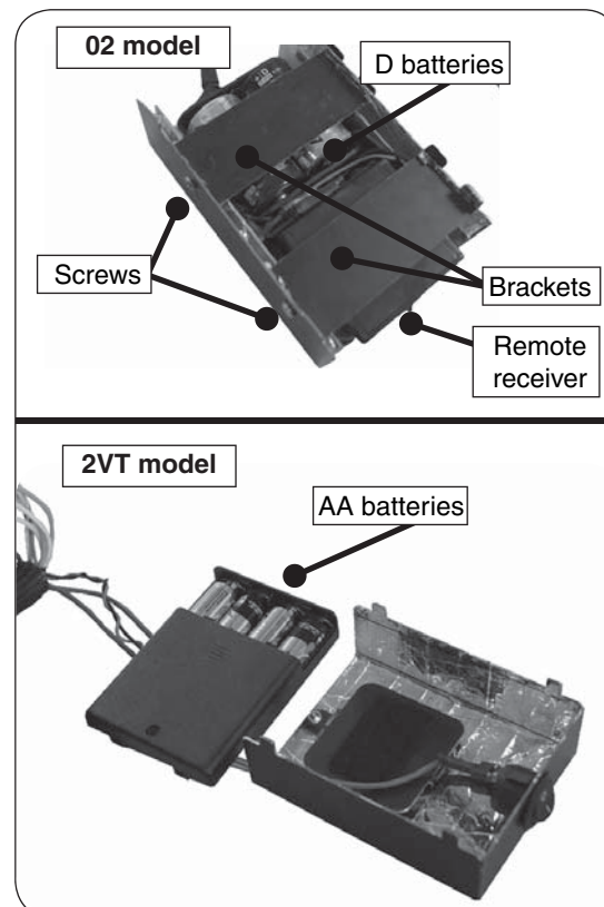
Fig. 22-3 Receiver/switch box batteries
